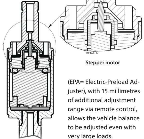
Touratech Suspension for BMW ESA
